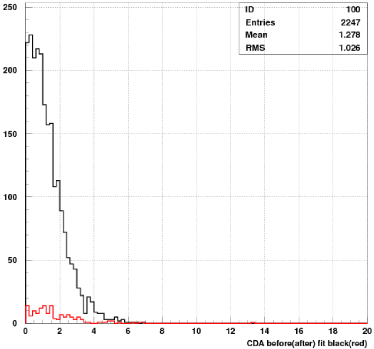
Least squares fit, Kpi2 decay, 4C fit MC, prob It 0.01
