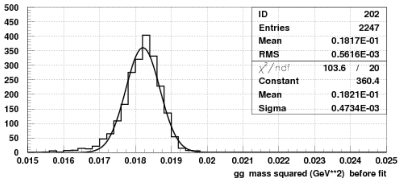
Least squares fit, Kpi2 decay, 4C fit MC, prob It 0.01
