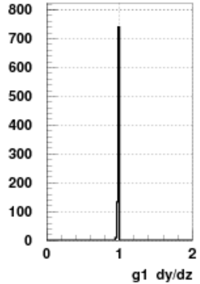
ratio fitted error to measured error, Kpi2 decay.
