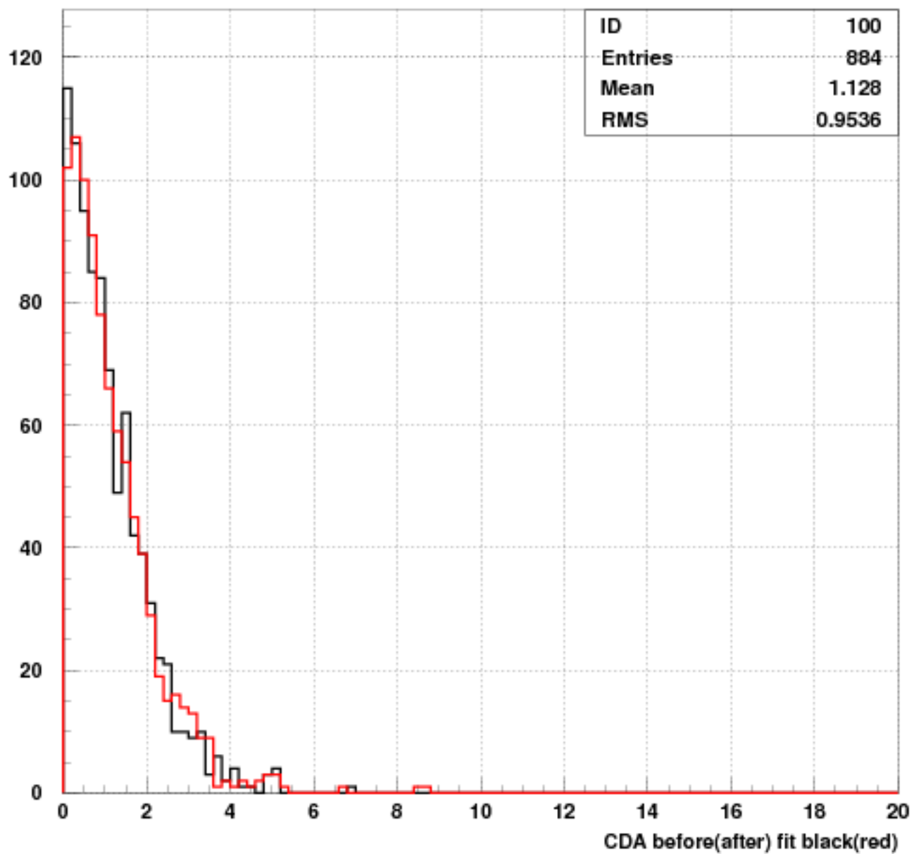
Least squares fit, Kpi2 decay, 4C fit DATA
