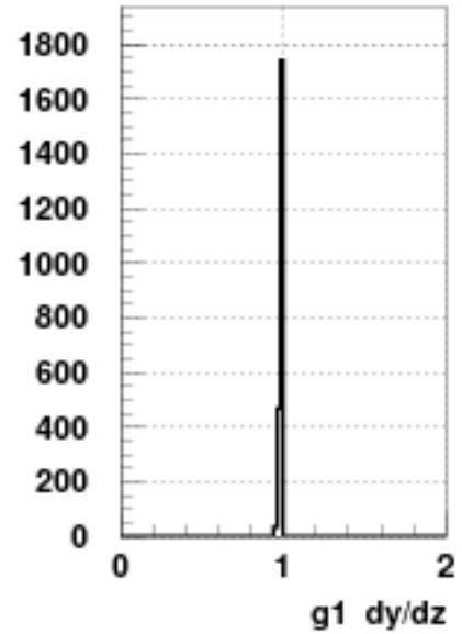
ratio fitted error to measured error, Kpi2 decay.
