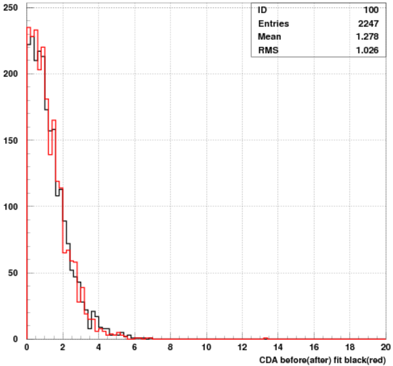
Least squares fit, Kpi2 decay, 4C fit MC
