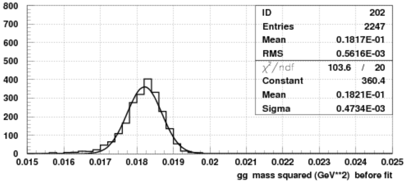
Least squares fit, Kpi2 decay, 4C fit MC
